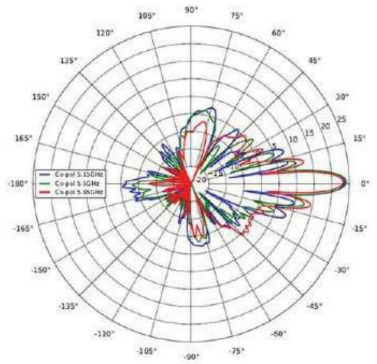
Elevation, Horizontal
