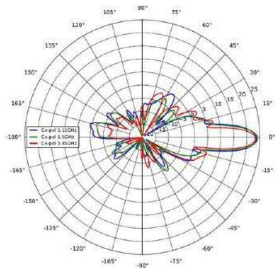
Azimuth, Horizontal
