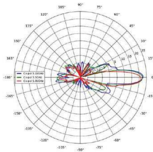
Elevation, Vertical
