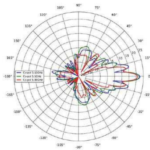
Azimuth, Vertical
